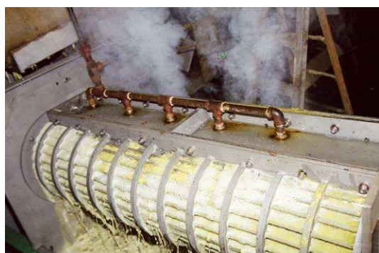
STEAM INJECTION IN TWIN SCREW PRESS
